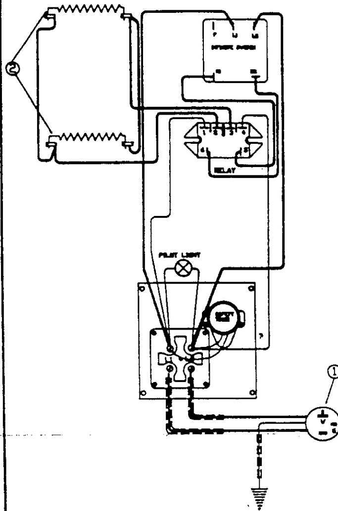
ELECTRICAL SCHEMATIC DB 609
