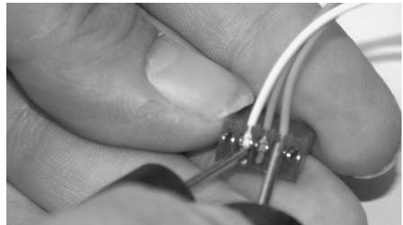
Input Test #2 with disconnected plug: Touch the voltmeter probes to the white and orange wires to test voltage going to the controller. The voltmeter must be in AC mode.
