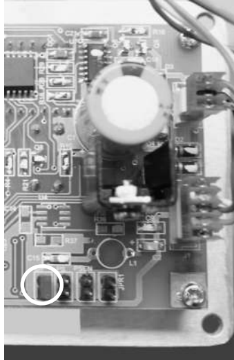
The C/F jumper terminal is on the back of the controller, circled above.
