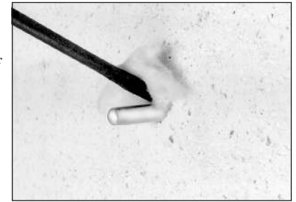
If the hole is 1/2" in diameter, stuff ceramic fiber around the protection tube.
